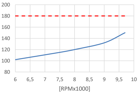
CHT [°C] - Under sparkplug sensor (ACC023/ACC024)
