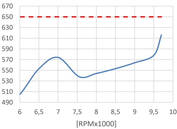
EGT [°C] - MY22 sensor (ACC025/ACC026)
